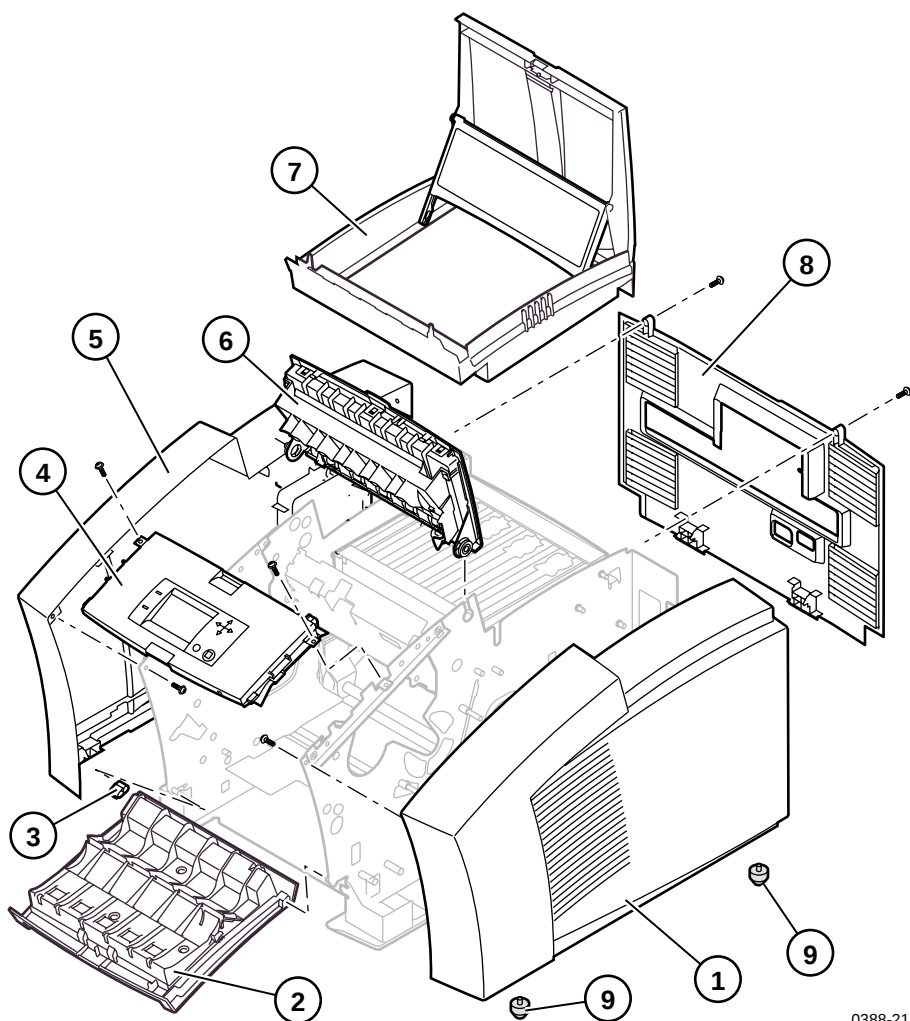
Figure 1 Cabinet FRUs
