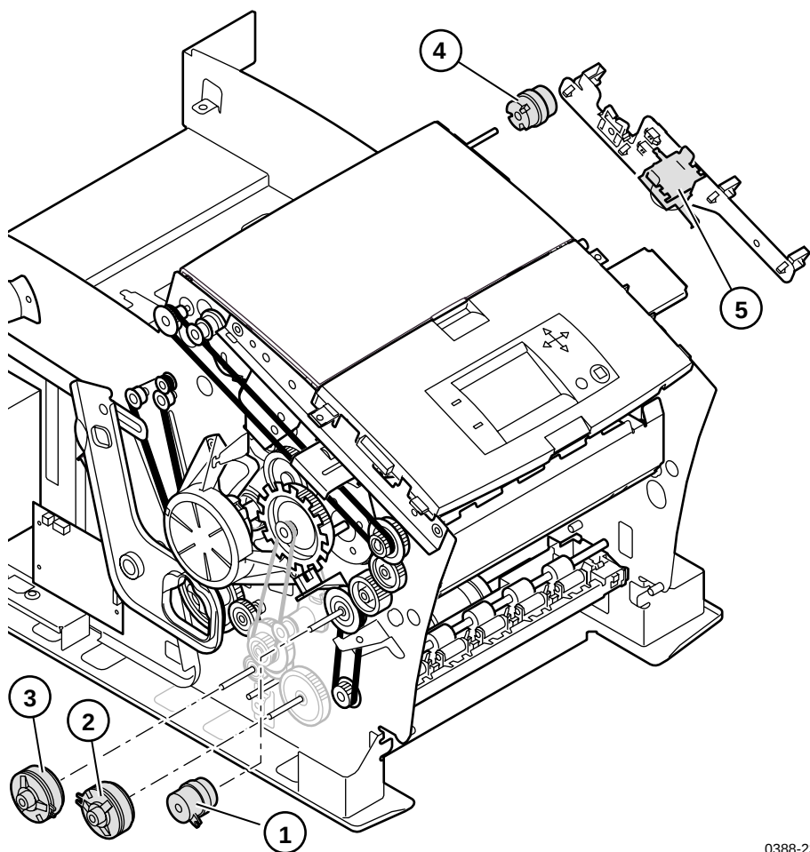
Figure 6 Solenoid and clutch FRUs
