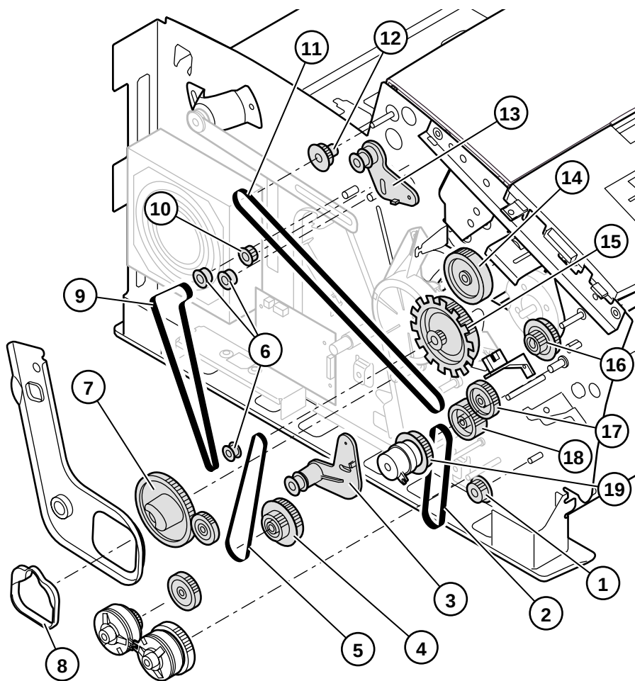
Figure 7 Gear and belt FRUs
