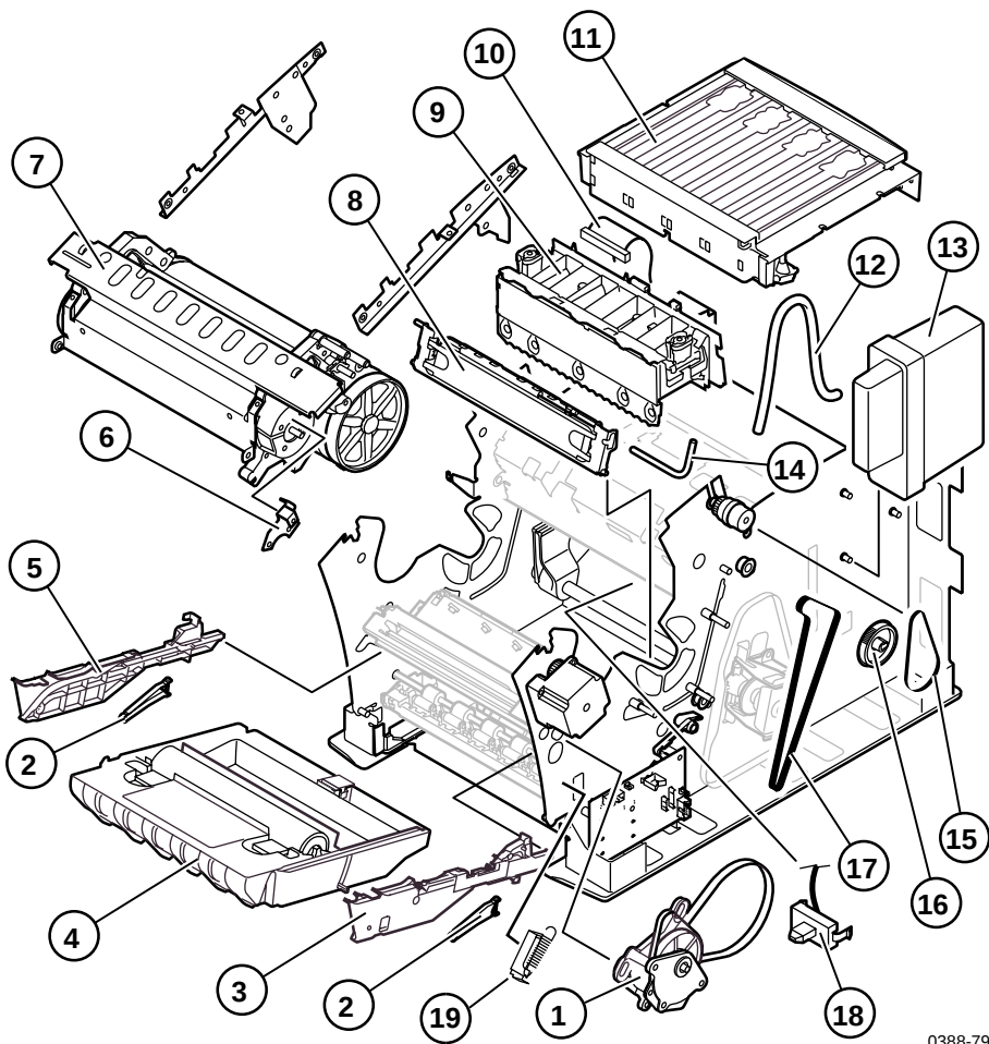
Figure 2 Imaging FRUs
