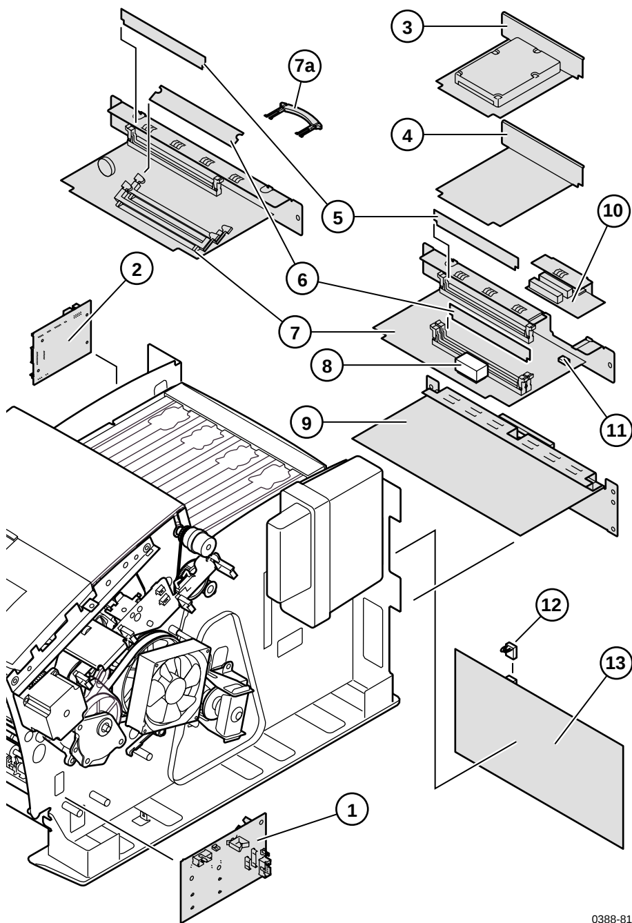
Figure 5 Circuit board FRUs
