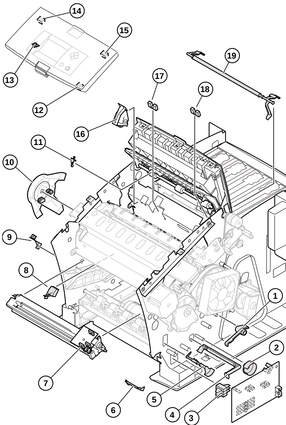
Figure 8 Sensor and flag FRUs
